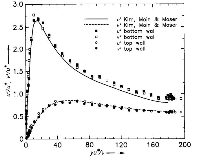
Fig. 5. Root-mean-square of the fluctuations in the streamwise, u' = (u^2)^{1/2} , and normal, v' = (v^2)^{1/2} , velocities
