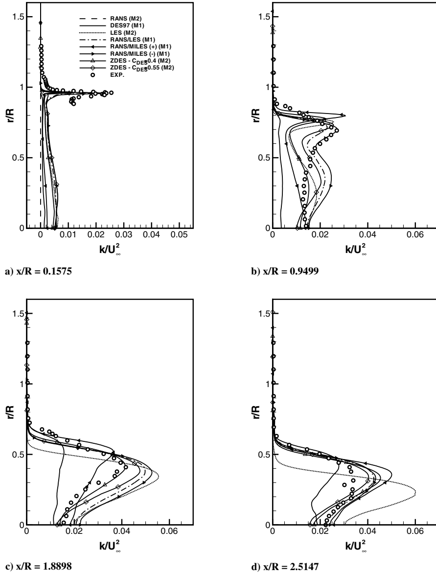
Fig. 11 TKE profiles.
