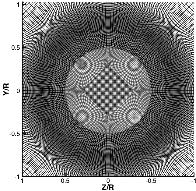
Fig. 2 Detailed view of M2 grid in the ( y - z ) plan near reattachment.
