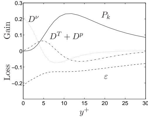
Figure 4.1: Flow between two parallel plates. Direct numerical simulations [23]. Re = U_C \delta / \nu = 7890 . u_* / U_C = 0.050 . Energy balance in k equation. Production P_k , dissipation \varepsilon , turbulent diffusion (by velocity triple correlations and pressure) D^T + D^p , and viscous diffusion D^\nu . All terms have been scaled with u_*^4 / \nu .
