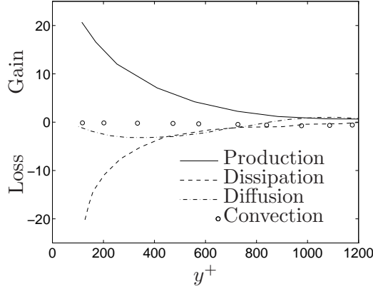
Figure 3.1: Boundary along a flat plate. Energy balance in k equation [45]. Re_\delta \simeq 4400 , u_*/U_0 \simeq 0.043 .
