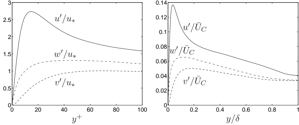
Figure 4.2: Flow between two parallel plates. Direct numerical simulations [23]. Re = U_C \delta / \nu = 7890 . u_* / U_C = 0.050 . Fluctuating velocity components u'_i = \sqrt{u_i'^2} .
