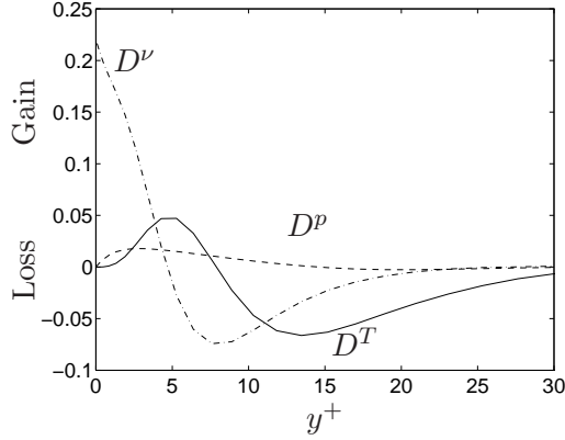
Figure 4.3: Flow between two parallel plates. Direct numerical simulations [23]. Re = U_C \delta / \nu = 7890 . u_* / U_C = 0.050 . Energy balance in k equation. Turbulent diffusion by velocity triple correlations D^T , Turbulent diffusion by pressure D^p , and viscous diffusion D^\nu . All terms have been scaled with u_*^4 / \nu .
