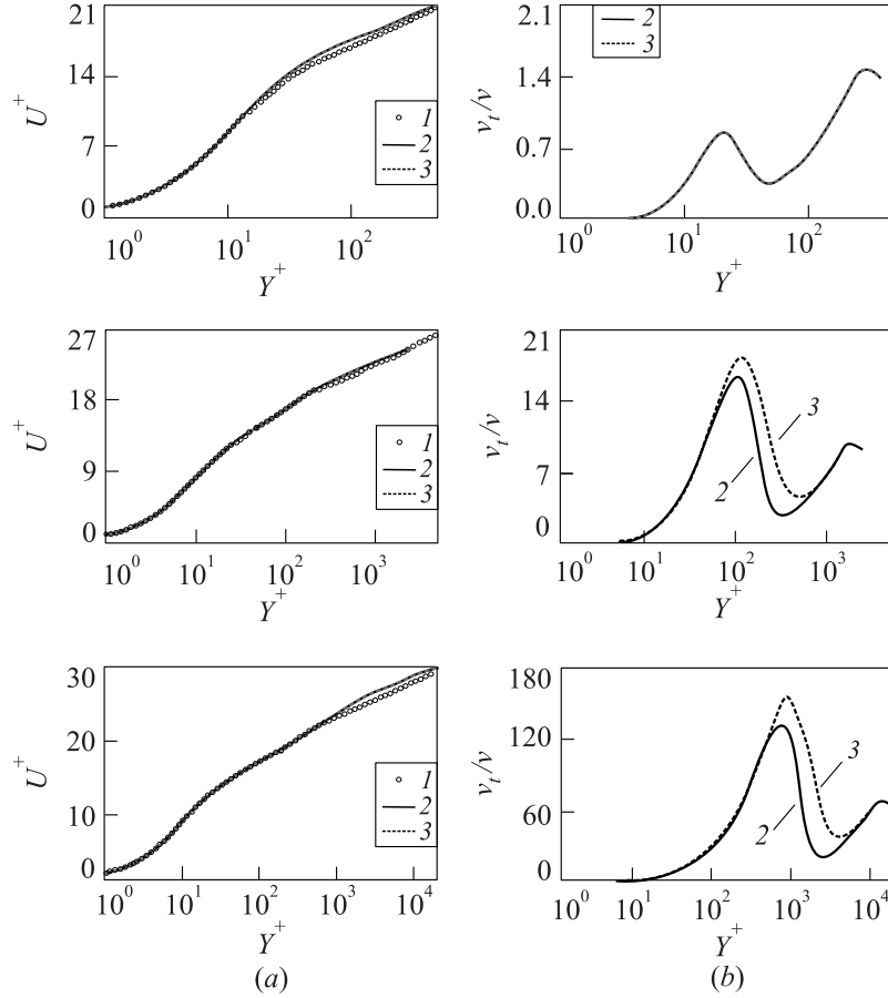
Figure 6 Effect of constant C_{dt1} on the SST IDDES of the developed channel flow: velocity (a) and eddy viscosity (b) profiles at different Reynolds numbers: upper row — Re_\tau = 395 ; middle row — 2400 ; and lower row — 18,000 ; 1 — correlation; 2 — IDDES, C_{dt1} = 8 ; and 3 — IDDES, C_{dt1} = 20
