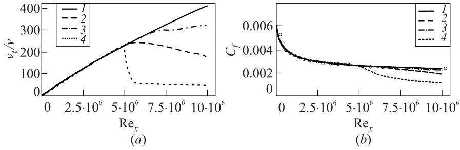
Figure 4 Effect of constant C_{d1} on the flat plate flow predicted by SST-based DDES: (a) distribution of eddy viscosity maximum value in each profile over the plate, and (b) distribution of skin friction coefficient distribution over the plate; 1 — SST; 2 — DDES, C_{d1} = 8 ; 3 — DDES, C_{d1} = 20 ; 4 — DES; and signs — experiment
