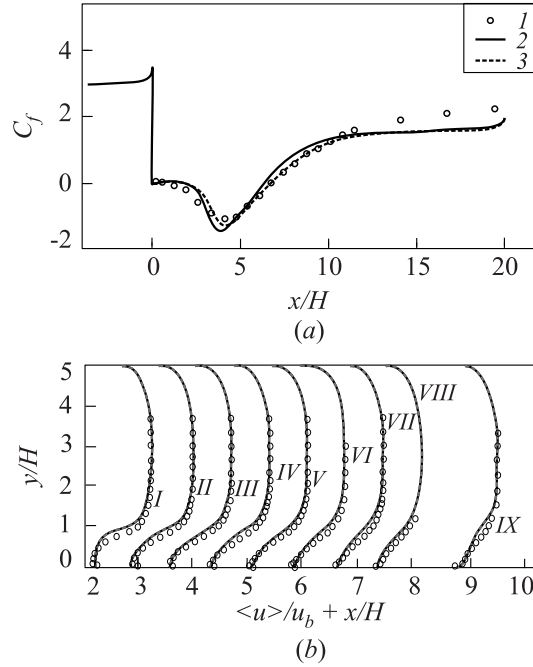
Figure 5 Effect of constant C_{d1} on the BFS mean flow predicted by SST-based DDES: (a) skin friction coefficient distribution over the step-wall and (b) profiles of streamwise velocity \langle u \rangle . Profiles are plotted at x/H = 2.2 (I), 3.0 (II), 3.7 (III), 4.5 (IV), 5.2 (V), 5.9 (VI), 6.7 (VII), 7.4 (VIII), and 8.7 (IX): 1 — experiment; 2 — DDES, C_{d1} = 8 ; and 3 — DDES, C_{d1} = 20
